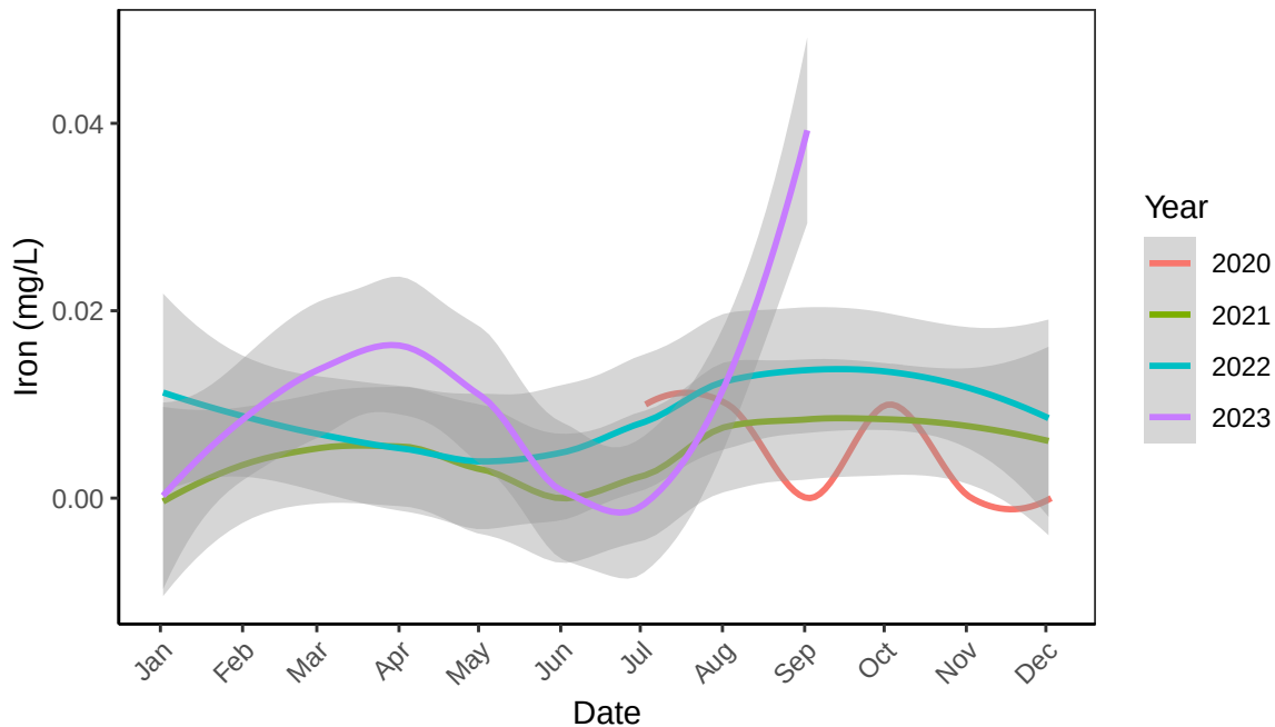
B2 Raceway 1 Iron (mg/L) Monthly Mean
